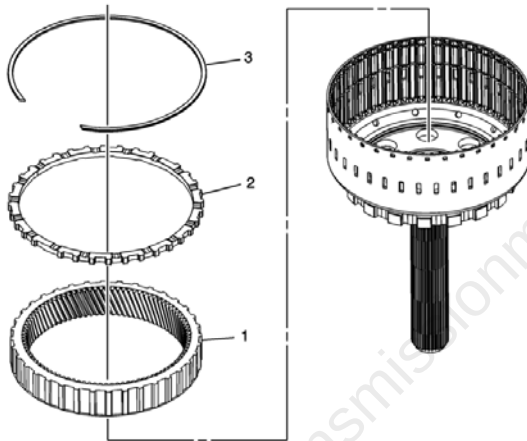
Output Shaft Assembly
